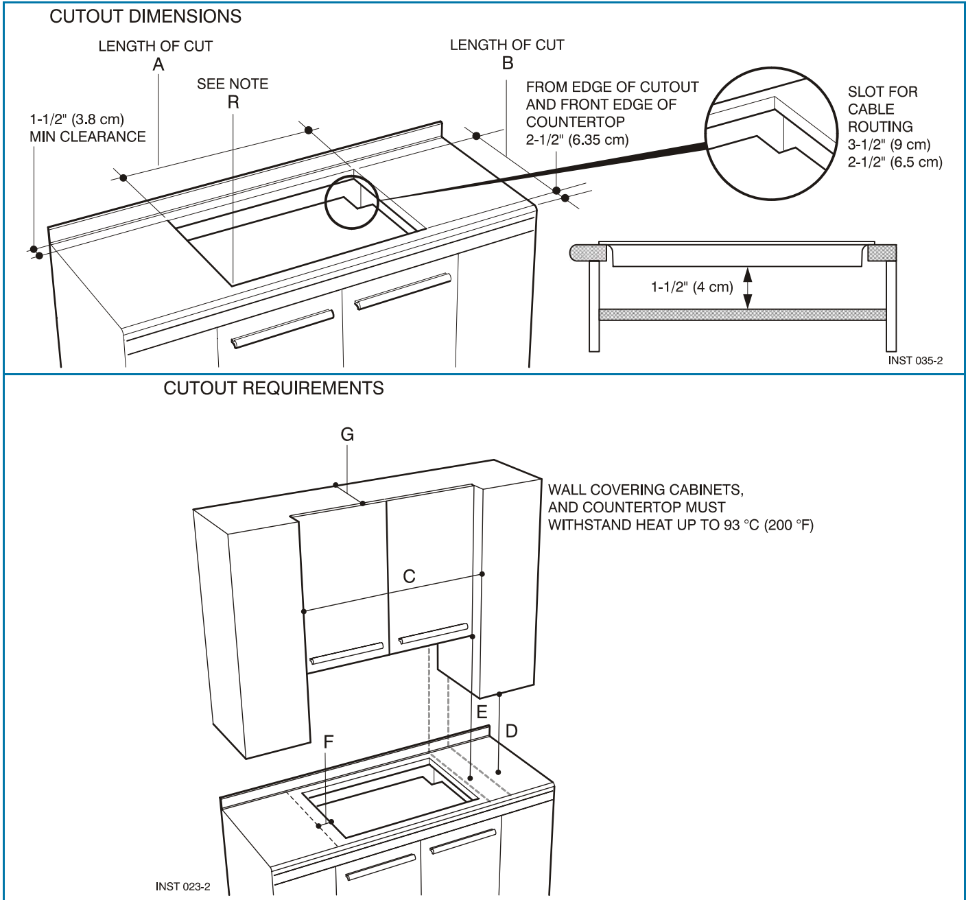
Figure 3. Cutout dimensions and requirements
